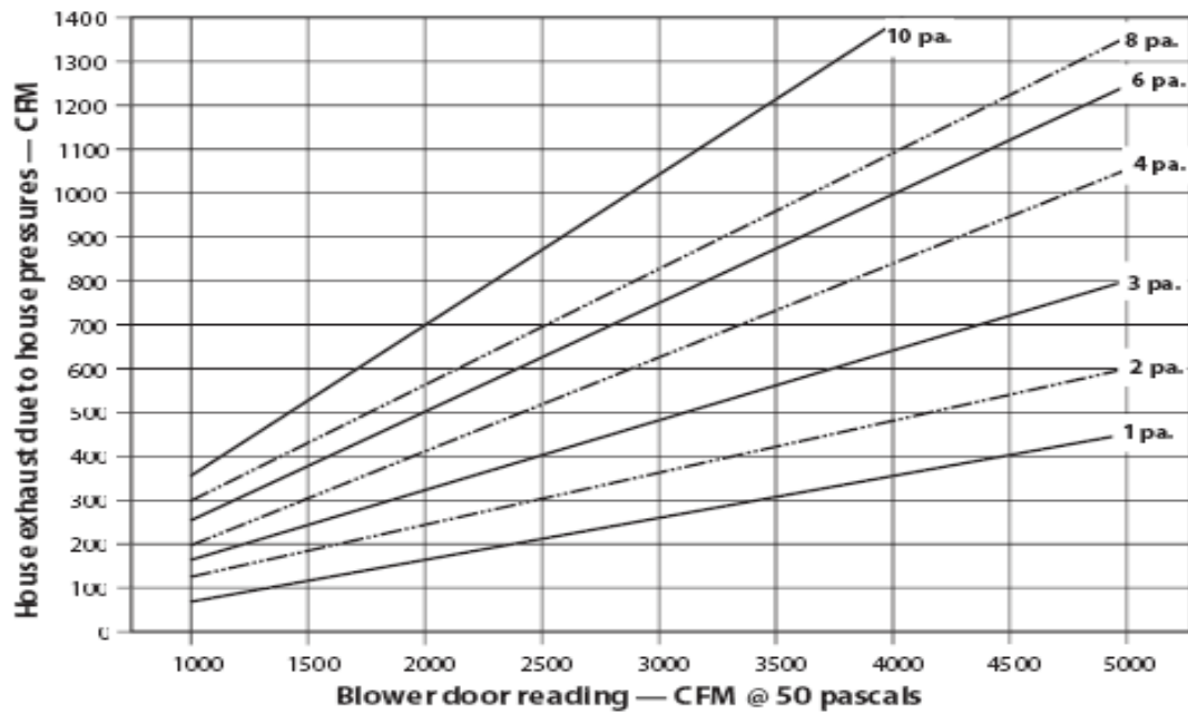
Chart 12-3 Depressurization Tightness Limit 14
